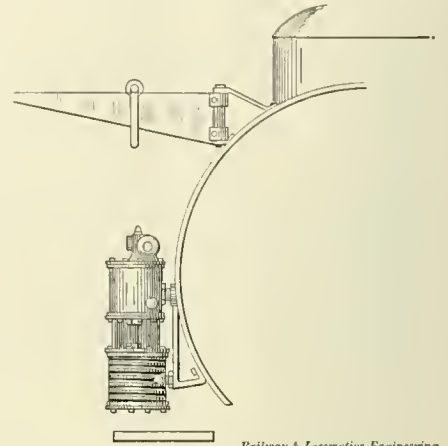
CRANE IN OPERATING POSITION.
